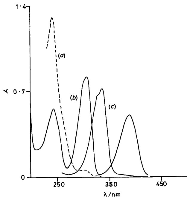
Figure 5. Absorption spectra in 19:1 v/v water-ethanol solutions of (a) TPB at pH 12.5; (b) TPBH + at pH 7.0; (c) TPBH 2 2+ at pH -0.5
