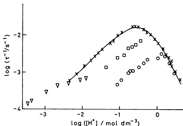
Figure 2. Log 1/\tau vs. log [H^+] for the hydrolysis of TPB in 19:1 v/v water-ethanol ( \times ); TPB in 1:1 v/v water-ethanol ( \circ ); Me-TPB in 19:1 v/v water-ethanol ( \nabla ); Me-TPB in 1:1 v/v water-ethanol ( \square ). The curve is drawn according to eqn. (2)
