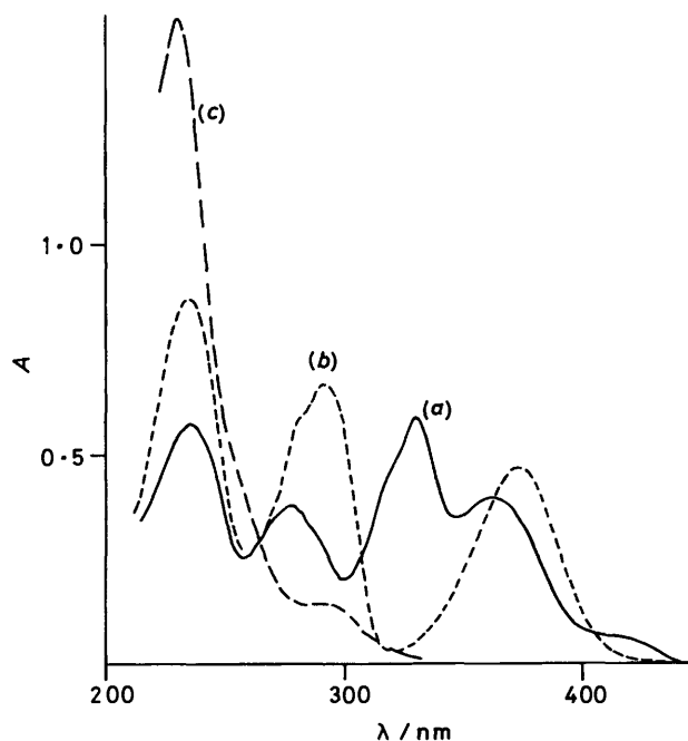
Figure 7. Absorption spectra in 19:1 v/v water-ethanol solutions of (a) DPPH + at pH 3.9; (b) DPP at pH 8.8; (c) DPP dep - at pH 11.9
